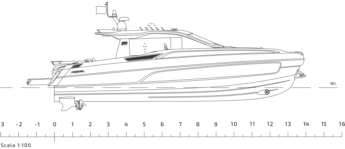
INBOARD PROFILE
